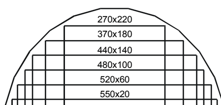
d=700 mm/30°
